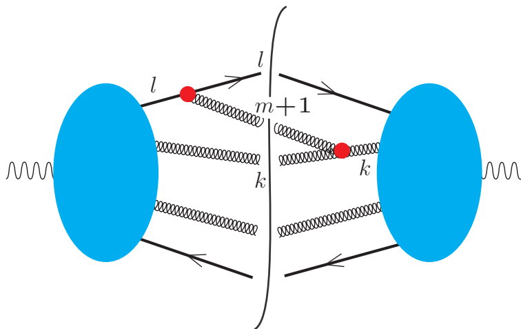
Figure 5. An interference graph contributing to \bar{w}_{lk} for a q \rightarrow q + g splitting.
