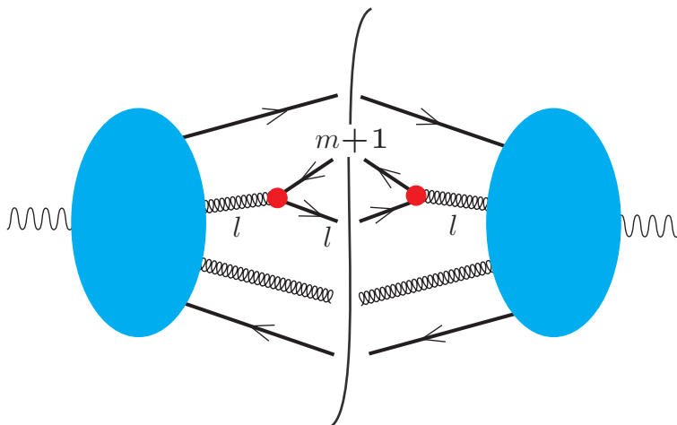
Figure 4. A graph contributing to \overline{w}_l for a g \rightarrow q + \bar{q} splitting.
