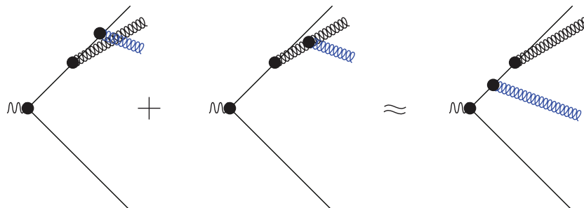
Figure 1. Emission of a soft gluon from a nearly collinear quark-gluon jet. The gluon is at a wider angle to the jet than the jet opening angle, but is very soft. The gluon does not resolve the jet, so the emission is as if the soft gluon were emitted from an on-shell massless parton moving in the direction of the jet and carrying the net color of the jet, as indicated on the right hand side of the approximation.
