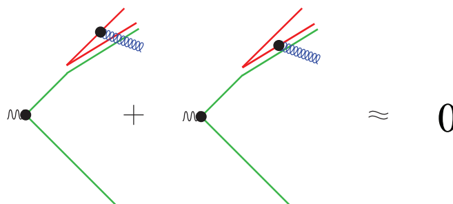
Figure 1. Emission of a soft gluon from a nearly collinear quark-gluon jet. The gluon is at a wider angle to the jet than the jet opening angle, but is very soft. The gluon does not resolve the jet, so the emission is as if the soft gluon were emitted from an on-shell massless parton moving in the direction of the jet and carrying the net color of the jet, as indicated on the right hand side of the approximation.
