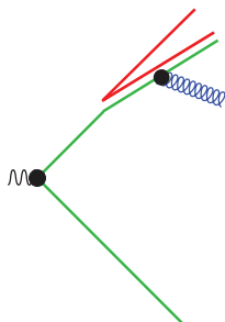
Figure 3. Emission of a soft gluon from a nearly collinear quark-gluon jet when the gluon in the jet is considered as \mathbf{3} \otimes \bar{\mathbf{3}} state. Emission from the part of the gluon that makes part of a wide angle dipole remains.
